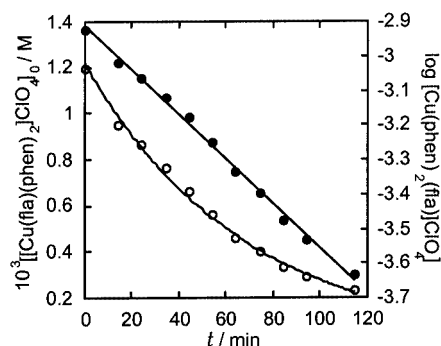
Figure 1. Time course for the oxygenation of [\text{Cu}(\text{phen})_2(\text{fla})]\text{ClO}_4 in DMF (○) and plot of \log\{[\text{Cu}(\text{phen})_2(\text{fla})]\text{ClO}_4\} (●) vs. reaction time for the oxygenation of [\text{Cu}(\text{phen})_2(\text{fla})]\text{ClO}_4 ( \{[\text{Cu}(\text{phen})_2(\text{fla})]\text{ClO}_4\}_0 = 1.35 \times 10^{-3} \text{ M} , [\text{O}_2] = 6.1 \times 10^{-3} \text{ M} , 120 °C).
