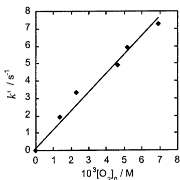
Figure 7. Plot of pseudo-first-order rate constant k' vs. \text{O}_2 pressure
