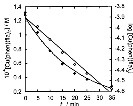
Figure 6. Time course for the oxygenation of \text{Cu}(\text{phen})(\text{fla})_2 in DMF ( \blacklozenge ) and plot of \log[\text{Cu}(\text{phen})(\text{fla})_2] ( \square ) vs. reaction time for the oxygenation of \text{Cu}(\text{phen})(\text{fla})_2
