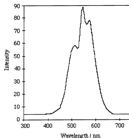
Figure 4. Electron spectrum of the emitted light during the oxygenation of \text{Cu}(\text{phen})(\text{fla})_2 in \text{DMF}
