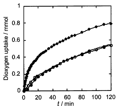
Figure 3. Time course for the oxygenation of the complexes \text{Cu}(\text{L})(\text{fla})_2 ( \text{L} = \text{phen} ( \blacklozenge ), \text{bpy} ( \bullet ), \text{TMEDA} ( \circ ); [\text{Cu}(\text{L})(\text{fla})_2]_0 = 0.4 \text{ mmol} in 50 \text{ mL} of \text{DMF} , [\text{O}_2] = 6.91 \times 10^{-3} \text{ M} , 80^\circ \text{C} )
