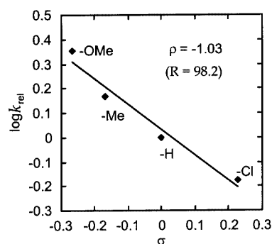
Figure 8. Hammett plot for the oxygenation of \text{Cu}(\text{phen})(4'\text{R-fla})_2 complexes
