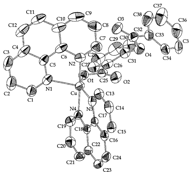
Figure 2. Molecular structure of [\text{Cu}(\text{phen})_2(O\text{-bs})]\text{ClO}_4 \cdot 1.5\text{CH}_2\text{Cl}_2
